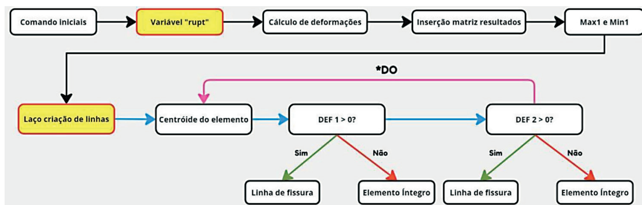
Figura 6 – Fluxograma do script.
