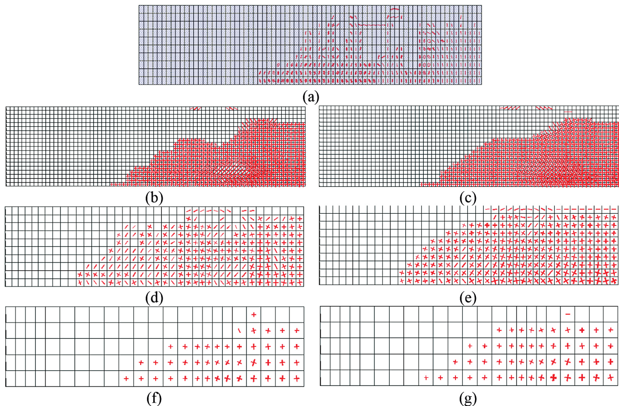
Figura 9 – Fissuras (a) S65_1_WW, (b) S186_1_C, (c) S186_1_B, (d) S186_2_C, (e) S186_2_B, (f) S186_4_C e (g) S186_4_B.
